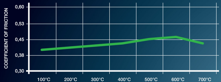
FRICION vs. TEMPERATURE RS 44
