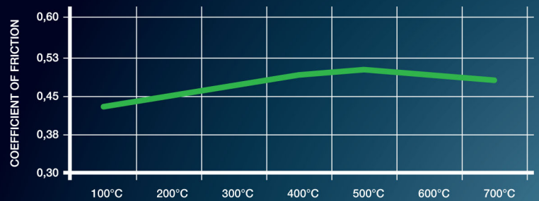
FRICION vs. TEMPERATURE RS 14
